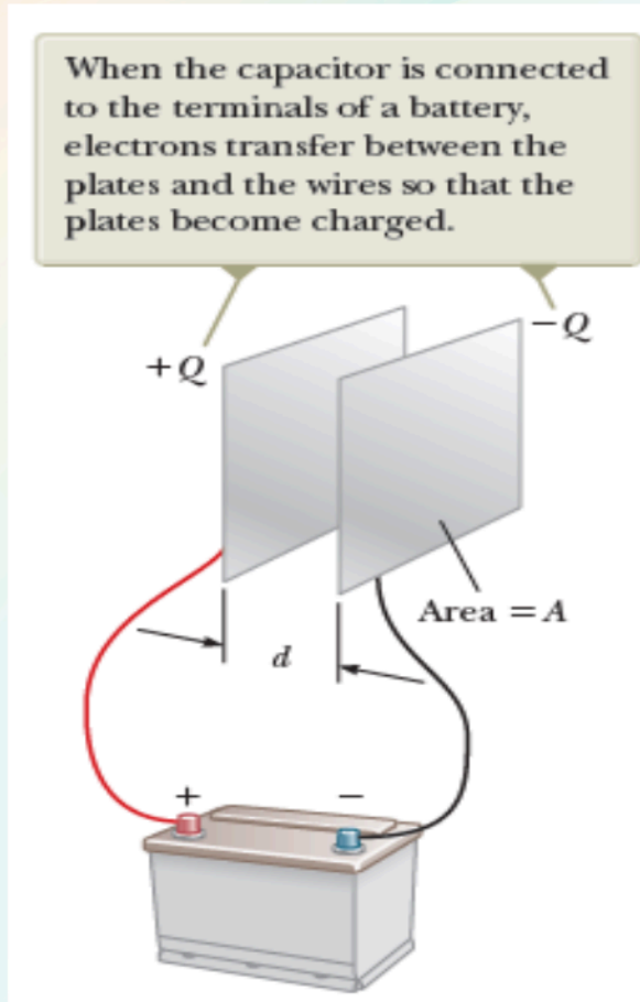
Figure 5. Parallel plate capacitor . From. Physics for Scientists and Engineers with Modern Physics (pp 778) by Serway, R. A., & Jewett, J. W. (2019). Australia: Cengage Learning.
