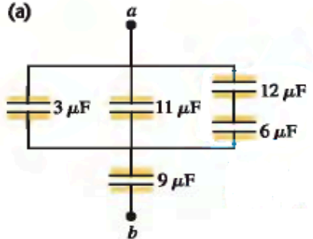
Figure 12. Capacitors in series and parallel. From: Sear's & Zemansky's University Physics With Modern Physics (pp 796) by Young, H. D., Freedman, R. A. & A. Lewis Ford(2016). England: Pearson
