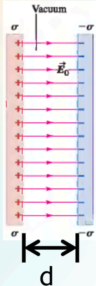
Figure 8. Electric Field Lines with Vacuum between Plates .. From. Sear's & Zemansky's University Physics With Modern Physics (pp 801) by Young, H. D., Freedman, R. A. & A. Lewis Ford(2016). England: Pearson.
