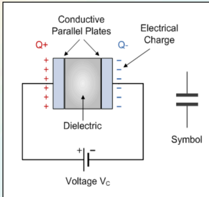
Figure 3. Conductive parallel plates. From https://www.electronics-tutorials.ws/wp-content/uploads/2018/05/capacitor-cap1.gif
