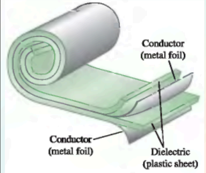
Figure 4. A common type of capacitor uses dielectric sheets to separate the conductors.. From. Sear's & Zemansky's University Physics With Modern Physics (pp 800) by Young, H. D., Freedman, R. A. & A. Lewis Ford(2016). England: Pearson.
