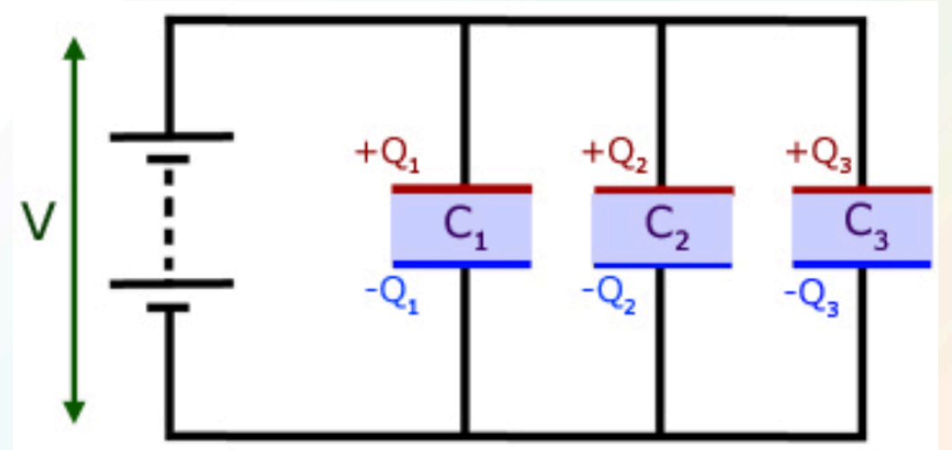
Figure11. Capacitors in parallel..From. https://tse3.mm.bing.net/th?id=OIP.90fBunwr_gzrkznVZBk1DCQAAAA&pid=Api&P=0&w=322&h=158
