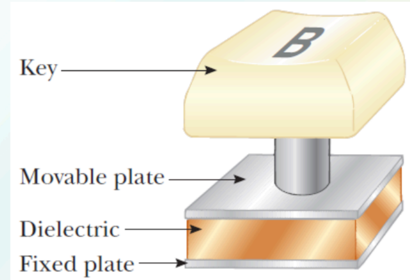
Figure 7. Computer Keyboard Button. From. Physics for Scientists and Engineers with Modern Physics (pp 780) by Serway, R. A., & Jewett, J. W. (2019). Australia: Cengage Learning.
